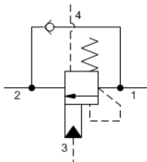
4-Port Vented, Non-adjustable
